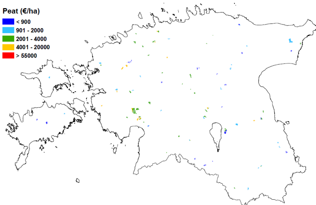
Figure 8. The ecosystem service provisioning areas and values of peat provisioning. The areas coloured from blue to red represent service provisioning areas according to the unit value (€/ha) supplied by ecosystem assets that was found by market price method. Areas coloured white represent areas (ecosystem assets) that do not supply the ecosystem service.
